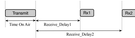
Figure 9: LoRaWAN node receive slot timing in Class-A mode of operation [2].
