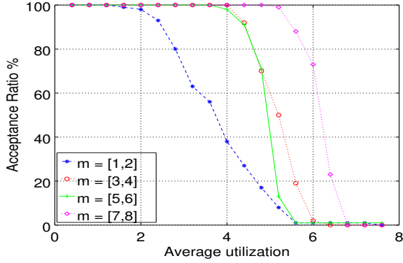
Fig. 3: Acceptance ratio for GEDF-VD in an 8-core platform under same ranges of degrees of parallelism.
